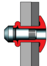
AFTER INSTALLATION
